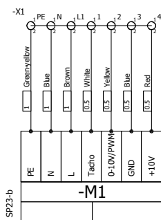
KF-T120 F 160 EC
