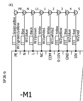
KF-T120 F 200 EC, KF-T120 F 250 EC, KF-T120 B 400 EC
